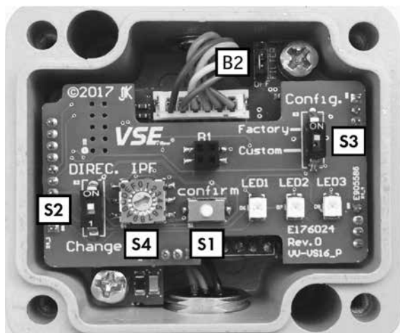
Fig. 4: Preamplifier peripheral board
