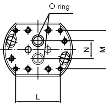
Cast iron version Connection diagram
